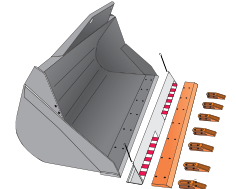
DIGGING BUCKET
